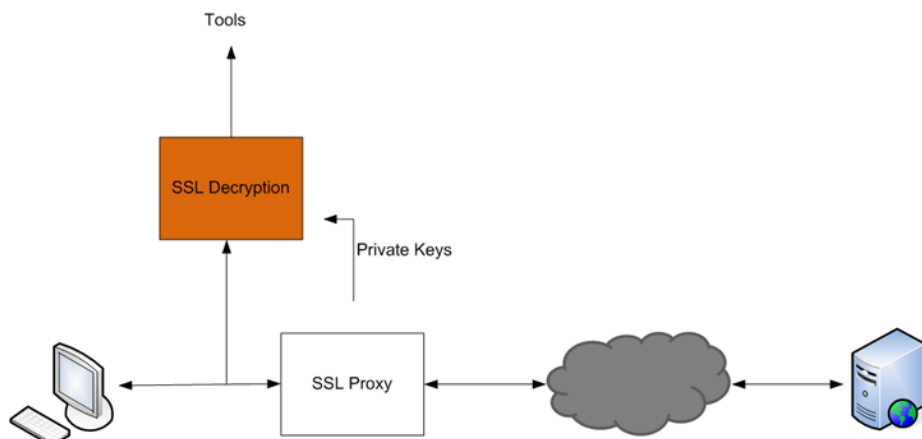
Figure 113 Outbound (Client/Enterprise Side)
