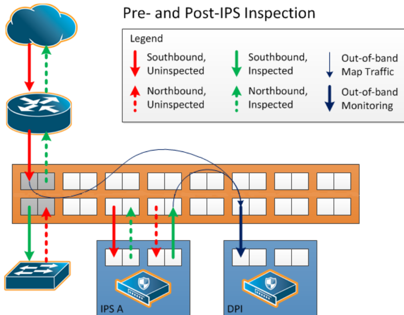
Figure 80 Out-of-Band Arrangement
