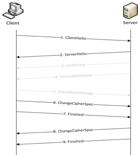
Figure 111 Resumed SSL Handshake
