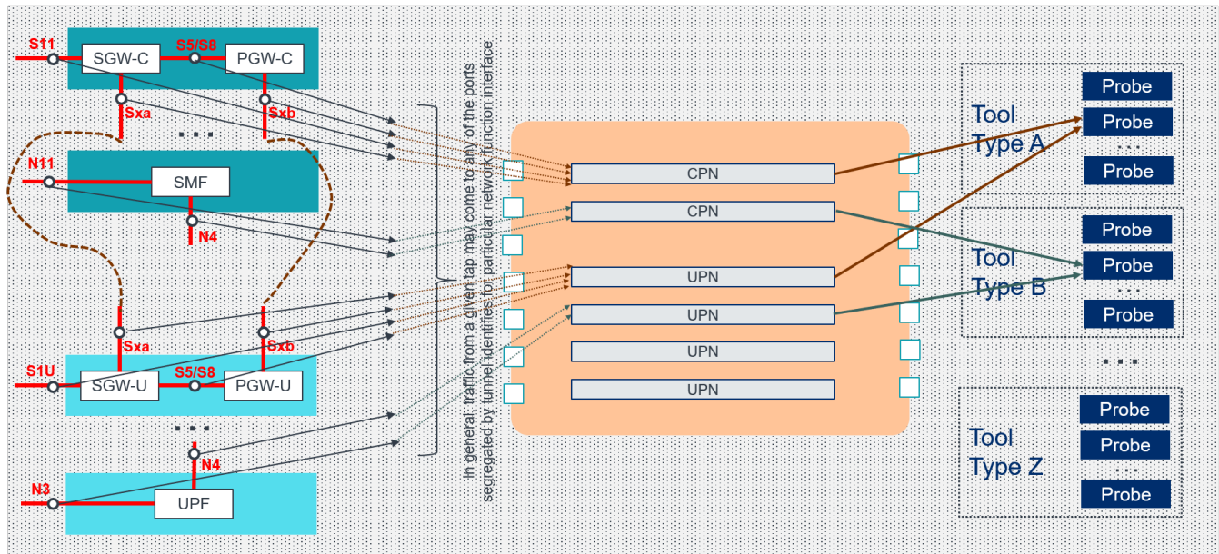
Figure 20 Traffic Correlation for LTE and 5G CUPS
