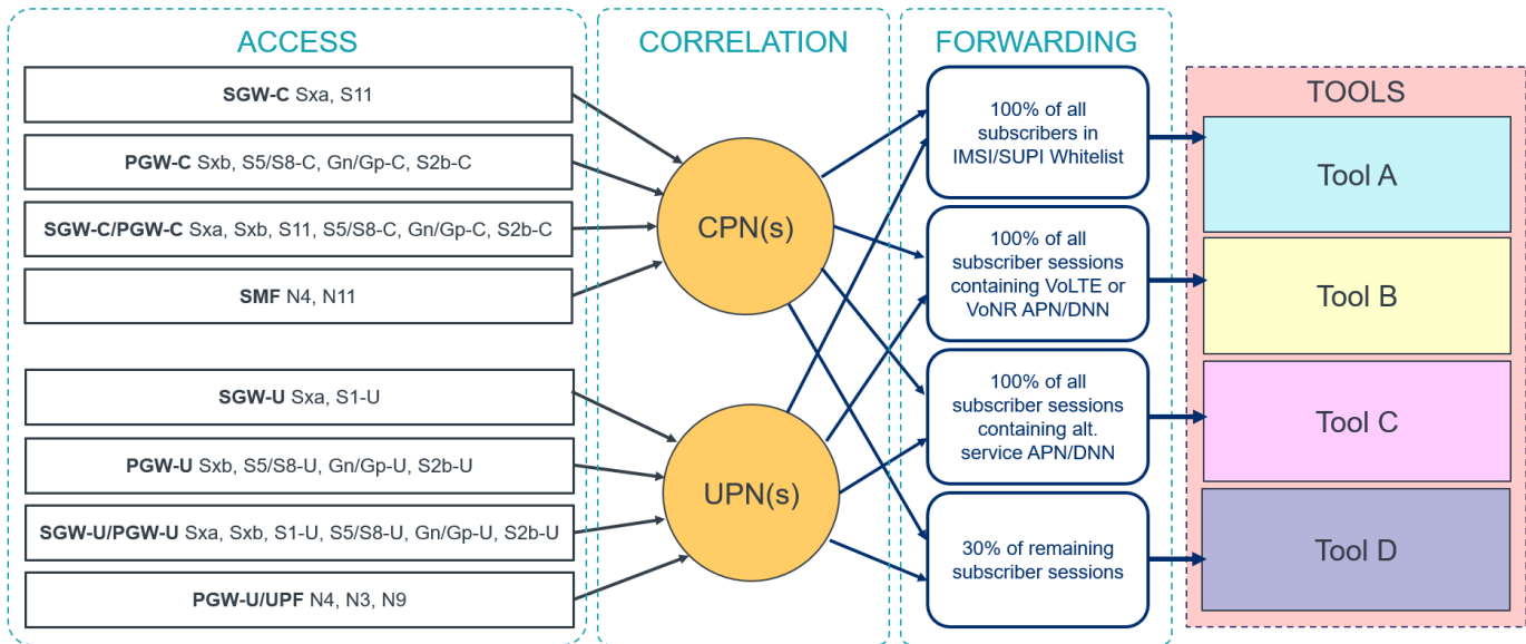
Figure 19 CUPS Traffic Visibility Solution
