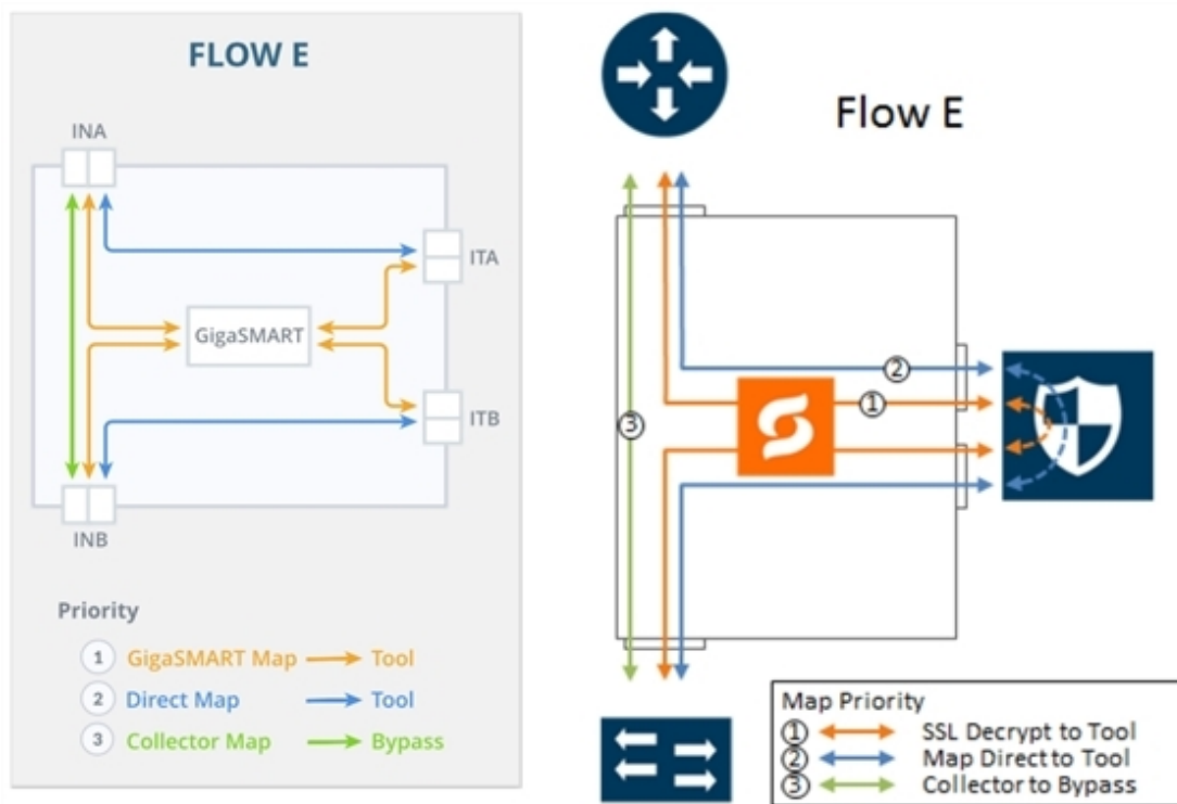
Figure 101 FLOW E Views
