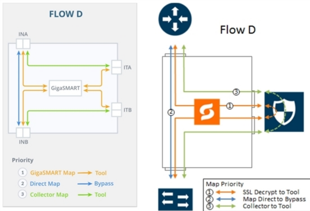
Figure 100 FLOW D Views
