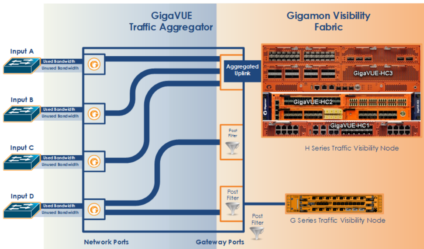
Figure 3 GigaVUE-FM-TA Packet Distribution
