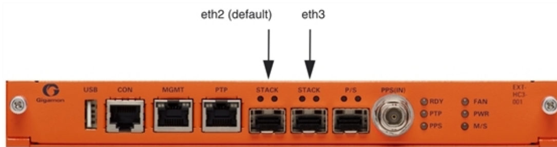
Figure 93 Stack Port Location on GigaVUE-HC3 Front
