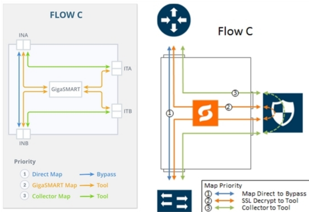
Figure 99 FLOW C Views
