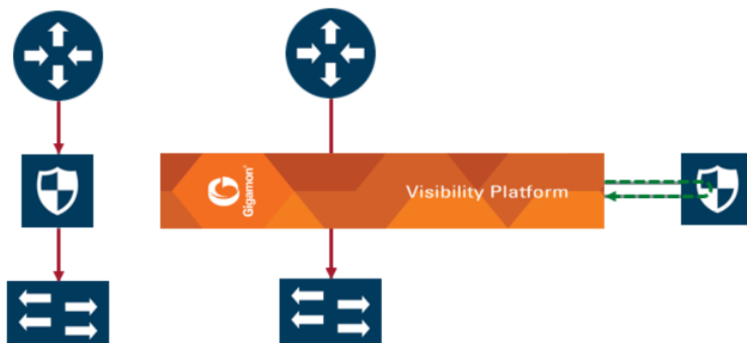
Figure 85 Simple Inline Tool Arrangement
