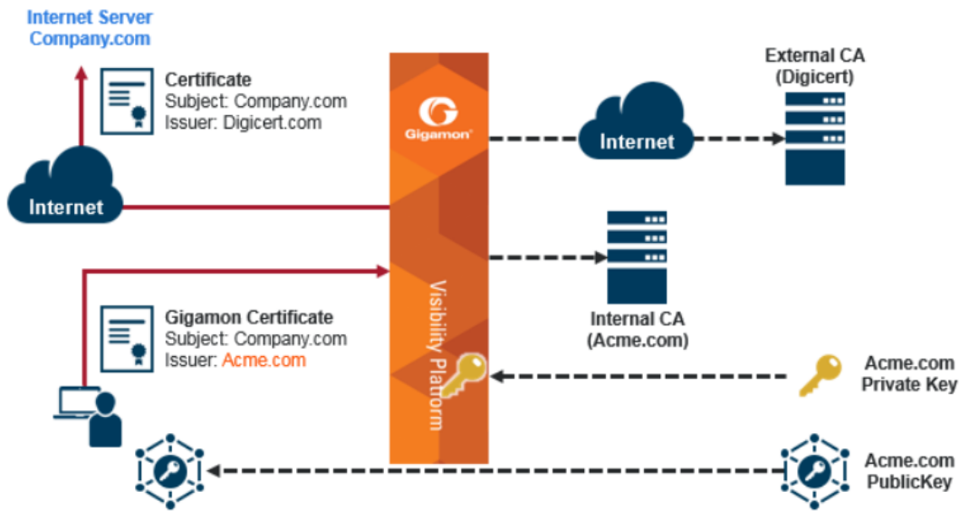
Figure 89 Outbound Deployment of Inline SSL Decryption
