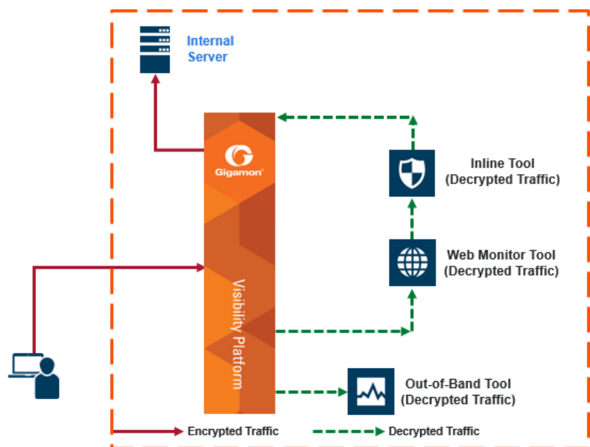
Figure 88 Inbound Deployment of Inline SSL Decryption
