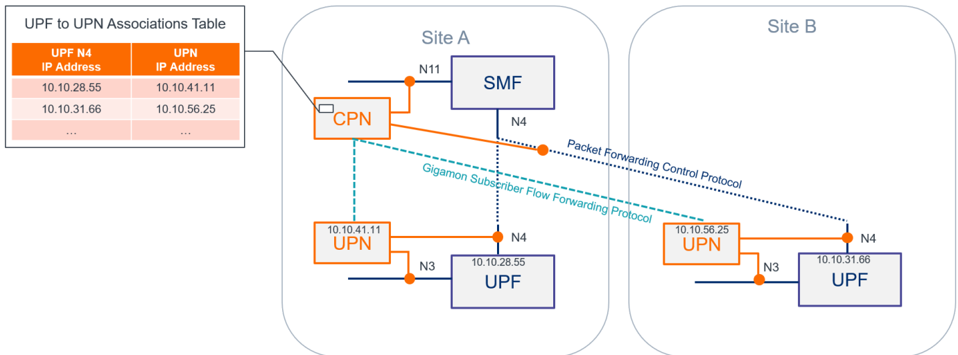
Figure 21 Dynamic CPN-to-UPN Mapping for 5G CUPS
