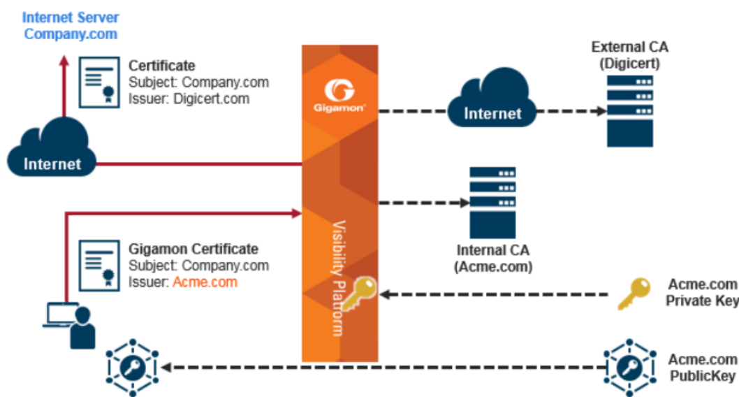
Figure 81 Outbound Deployment of Inline SSL Decryption
