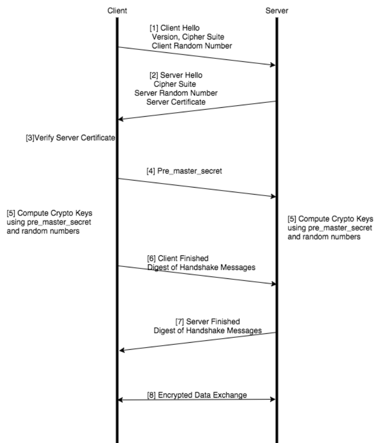
Figure 78 Basic SSL Handshake
