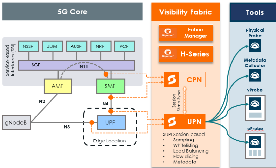
Figure 18 5G Stand Alone Packet Core Network
