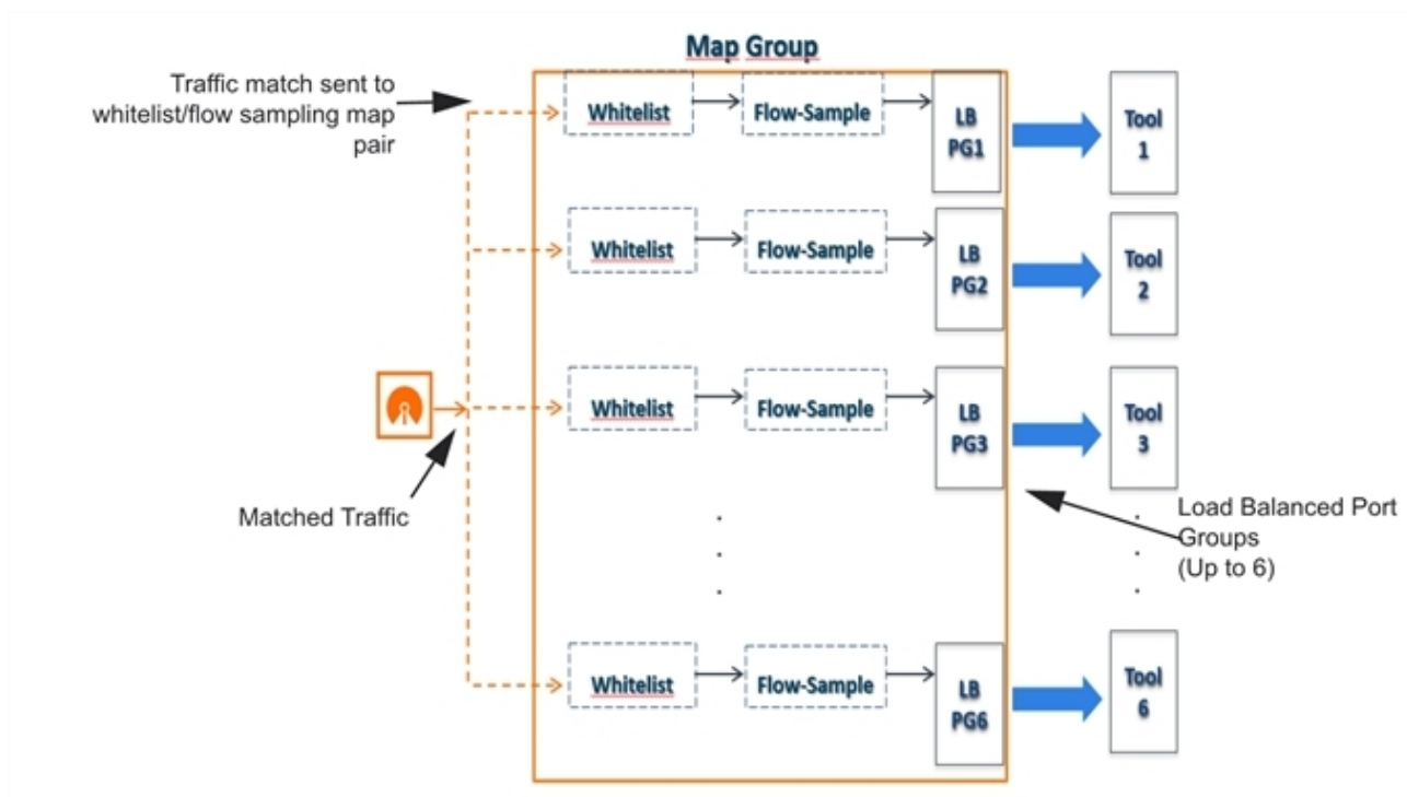
Figure 23 GTP Overlap Flow Sampling Map Groups
