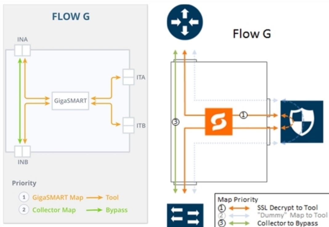
Figure 103 FLOW G Views
