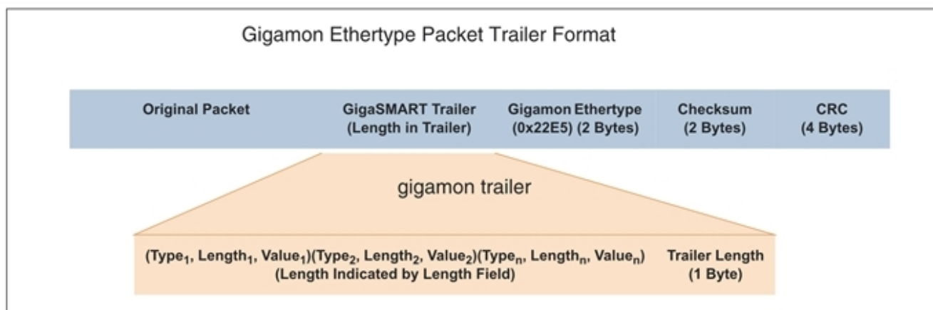
Figure 160 GigaSMART Trailer Format
