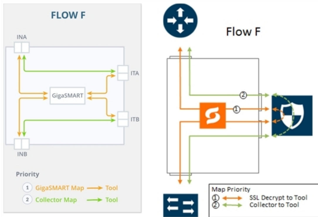
Figure 102 FLOW F Views
