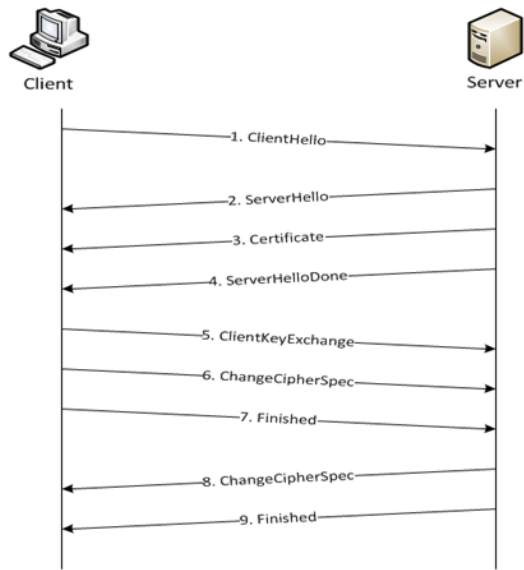
Figure 110 Basic SSL Handshake
