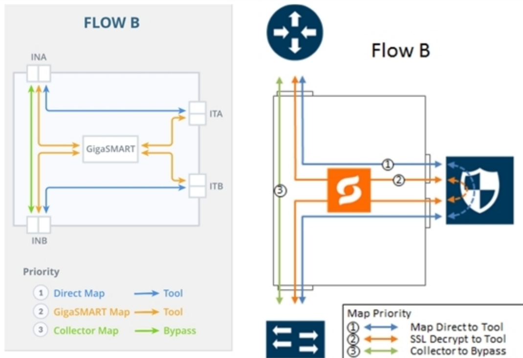
Figure 98 FLOW B Views
