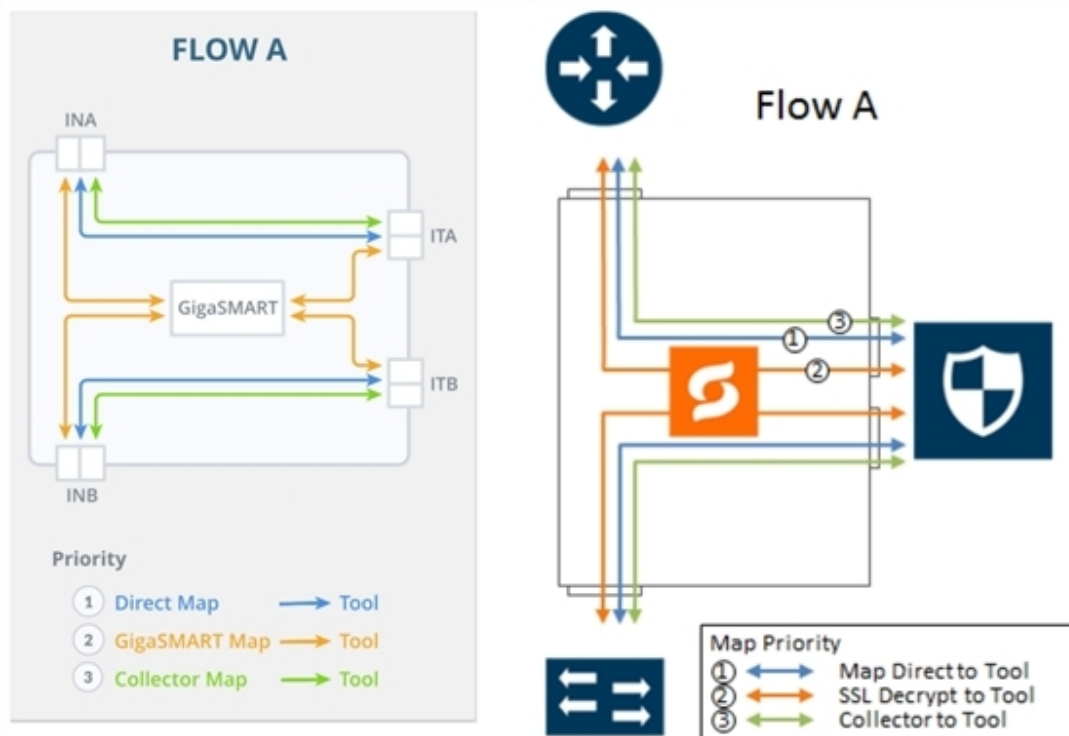
Figure 97 FLOW A Views
