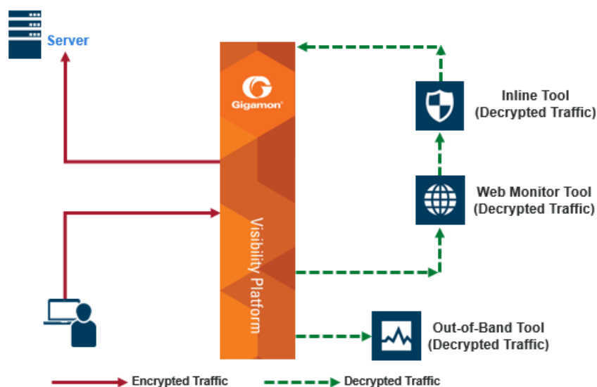
Figure 77 Inline SSL Decryption Example, Outbound
