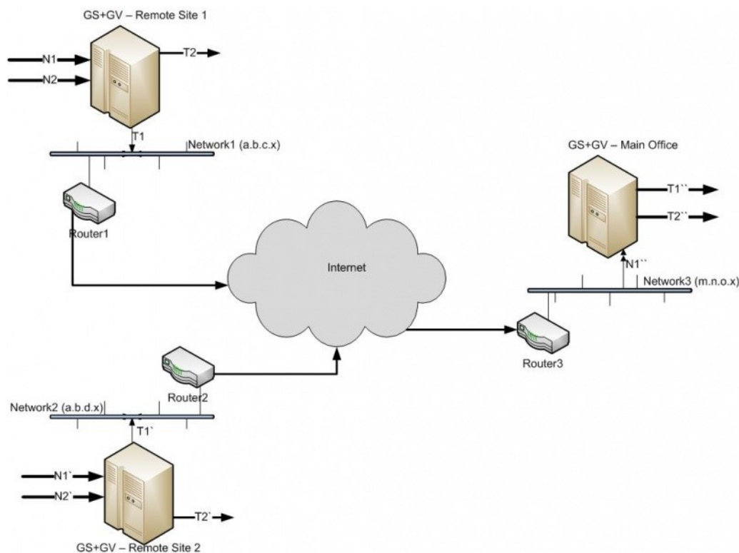
Figure 132 L2GRE Tunnel Encapsulation/Decapsulation
