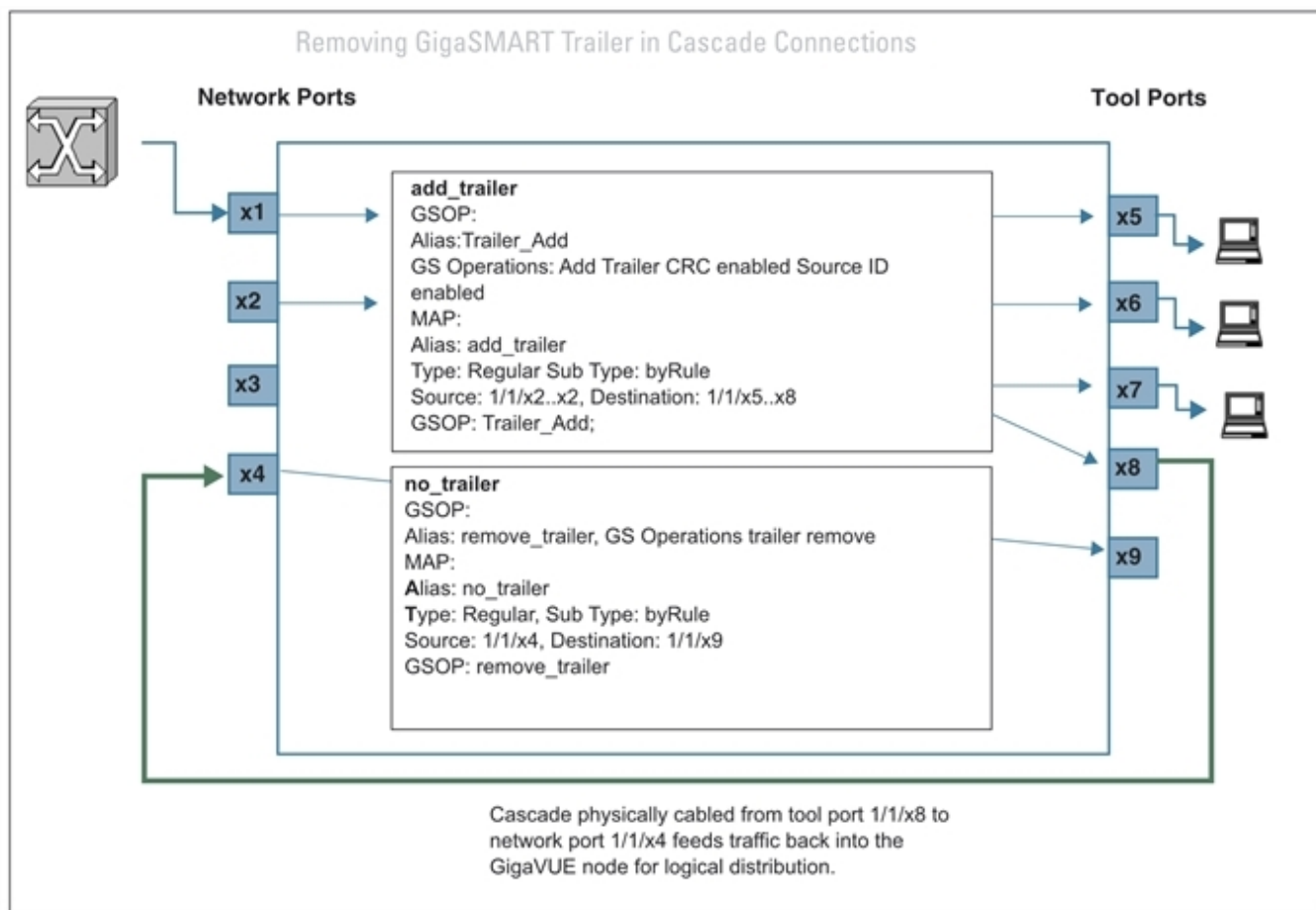
Figure 159 Removing the GigaSMART Trailer from a Cascade Connection
