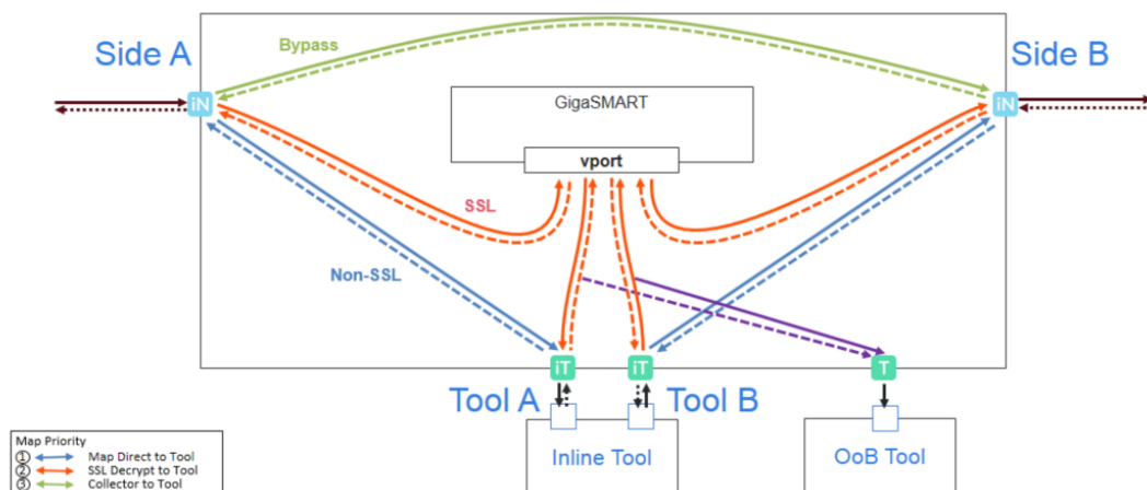
Figure 91 Packet Flow for Inline SSL Decryption
