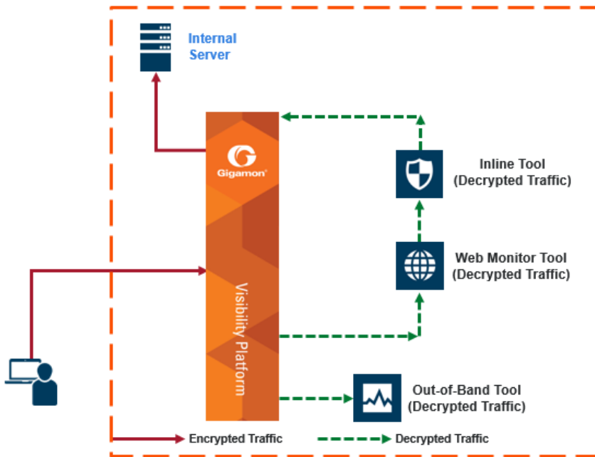
Figure 80 Inbound Deployment of Inline SSL Decryption
