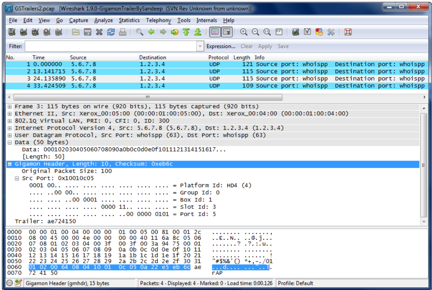
Figure 161 Wireshark Decode of GigaSMART Trailer
